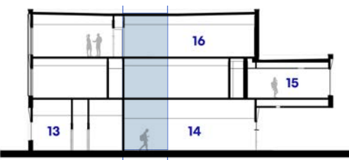
Cross Section 5
