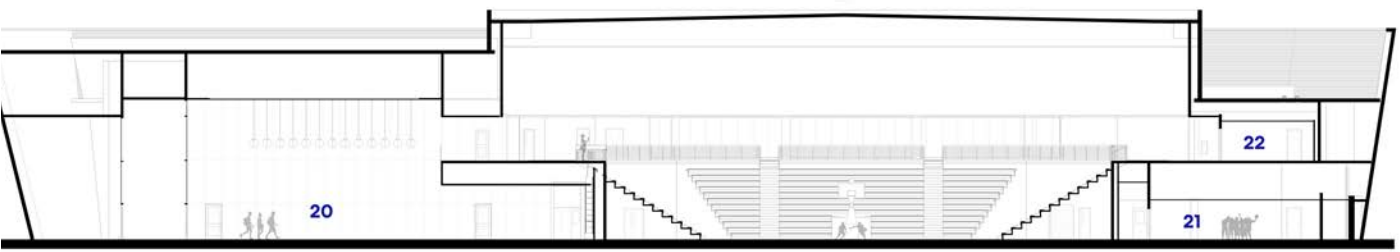
East-West Gymnasium Section 7
